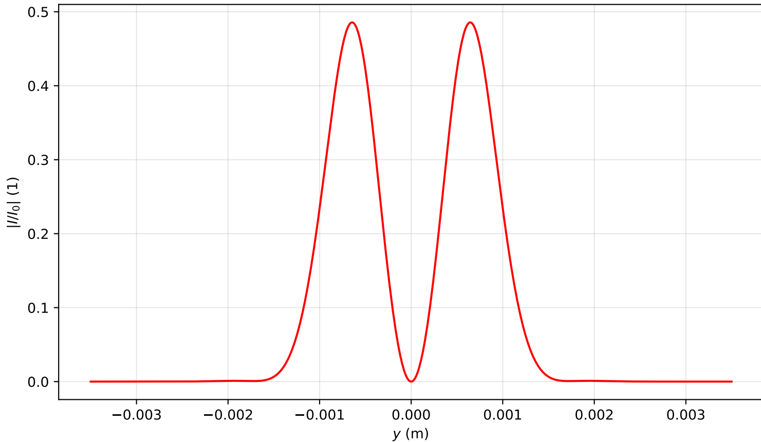
Intensity profile I(x=0, y, z=1.672)/I_0 , \text{Pin}=2.0\text{Pcr} , artificial time
